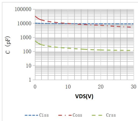
Fig.2 Capacitance Characteristics
